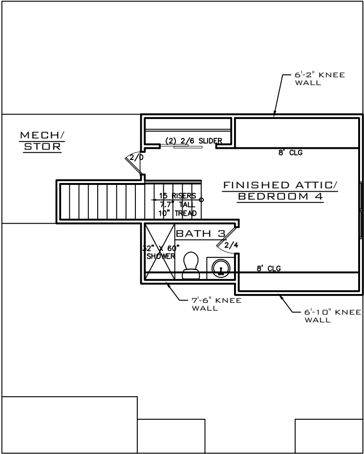
WALK UP ATTIC FLOOR PLAN
